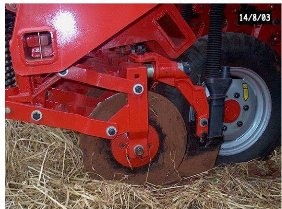
Fig. 7. A no-till seeder fitted with a fluted disk which can cut through the crop residue mulch and place seed in a narrow slot. The seed is covered by a press wheel that follows the slot opener.
