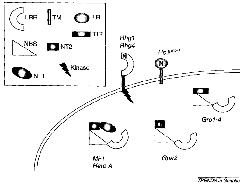
Figure 1. A comparison of predicted protein structure of the cloned nematode resistance gene products. The five protein structure classes of plant Nem- R genes are shown in their predicted cellular location. The yellow line represents the cell membrane and the grey area represents the cytoplasm. The Nem- R genes Mi-1 , Hero A , Gpa2 and Gro1-4 are predicted to be cytoplasmic, whereas Rhg1 , Rhg4 and Hs1 pro-1 are predicted to span the cell membrane. Protein motifs are shown in the key (upper left). Abbreviations: LR indicates a leucine rich region; TM, a transmembrane domain; LRR, a leucine rich repeat region; kinase, a protein kinase domain; NBS, a conserved motif containing a nucleotide binding site; TIR, toll-interleukin receptor-like domain; NT-1, amino terminal domain of NBS-LRR genes with long N-terminal regions; NT2, region immediately N-terminal to the NBS region of non-TIR NBS-LRR genes. The motif containing the letter N inside is at the amino terminus of the protein.
