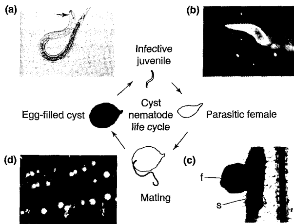
Figure 1. The life cycle of a plant parasitic cyst nematode. Key stages in the life cycle of a cyst nematode female are shown in the center. (a) Infective second stage juvenile (J2) with stylet indicated by arrow (photo courtesy of J. D. Eisenback and E.C. McGawley; www.mactode.com ). The J2 is ~ 0.4 mm in length. (b) The tail of a J2 (stained orange) can be seen as the nematode penetrates the plant root (adapted with permission from Ref. [33]). (c) An infected root, with a bulbous parasitic female (f), is shown on the left and an uninfected root is shown on the right (photo courtesy of J. D. Eisenback and U. Zunke, www.mactode.com ). The elongated syncytium (s) consists of plants cells that have fused together and serve as the feeding cell for the developing nematode. (d) Root sections with egg-filled cysts of Globodera rostochiensis (top root) and Globodera pallida (bottom root) appearing as golden or light colored globes, respectively, decorating the roots (photo courtesy of J. D. Eisenback and U. Zunke).
