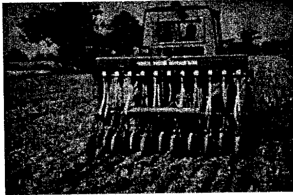
Fig. 2. The 2BMF-11 no-till wheat planter.
